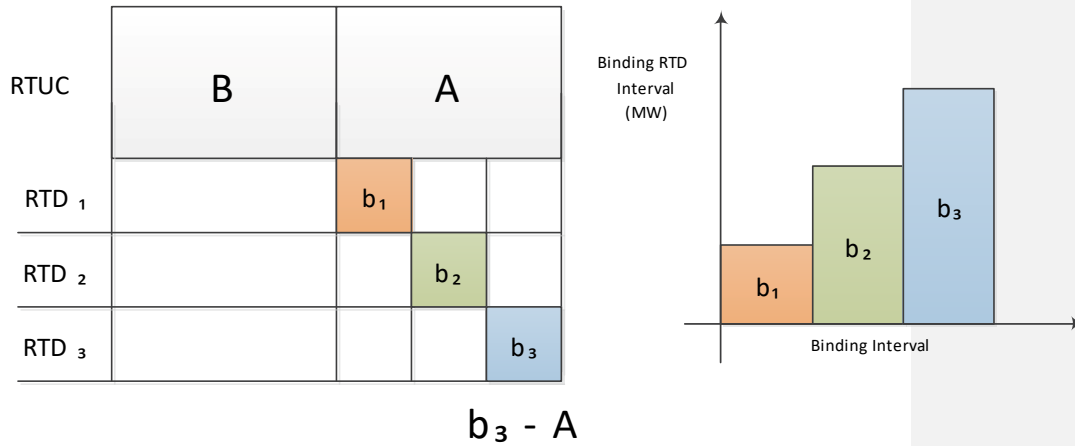
Figure 4: Histogram construction in FMM
