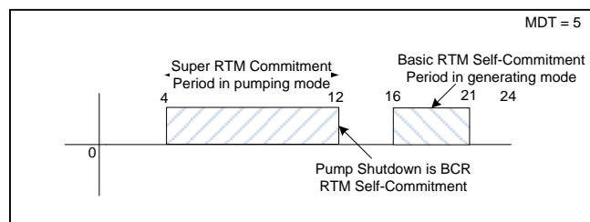
Figure 34: Illustration for Rule #33
